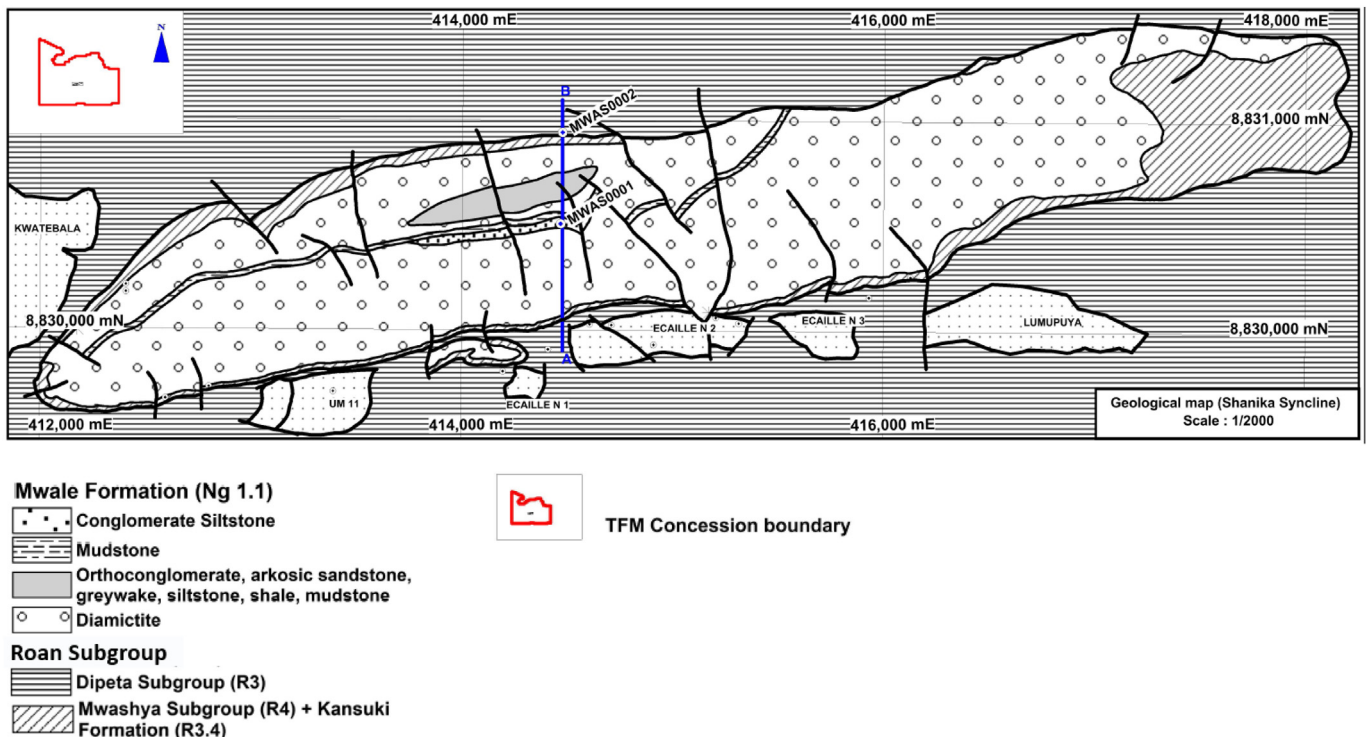
Fig. 2. Location of drill holes MWAS001 and MWAS002 in the Shanika syncline.
